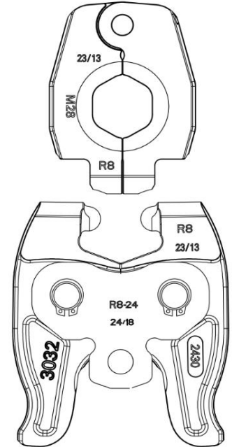
R8 Angle jaw with R8-24 rotating adaptor jaw
