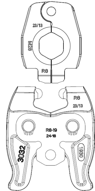
R8 Angle jaw with R8-19 rotating adaptor jaw
